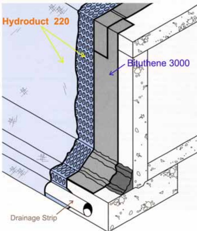
Hydroduct 220
